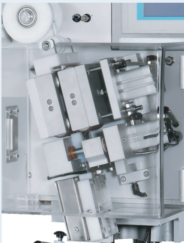
• Pouch Desiccant Cutting and Dispensing Mechanism
